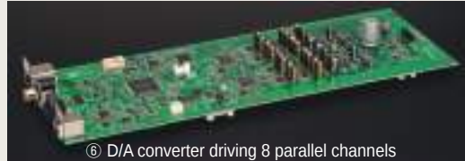
⑥ D/A converter driving 8 parallel channels
