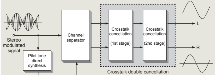
■ DS-DC Type Stereo Demodulator Circuit
