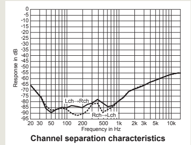
Channel separation characteristics
